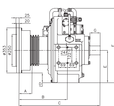
S Type Directly Mount
